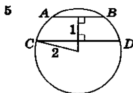
x = CD, AB = 2
